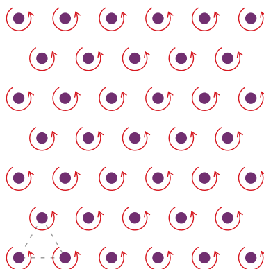
VORTEX LATTICE
