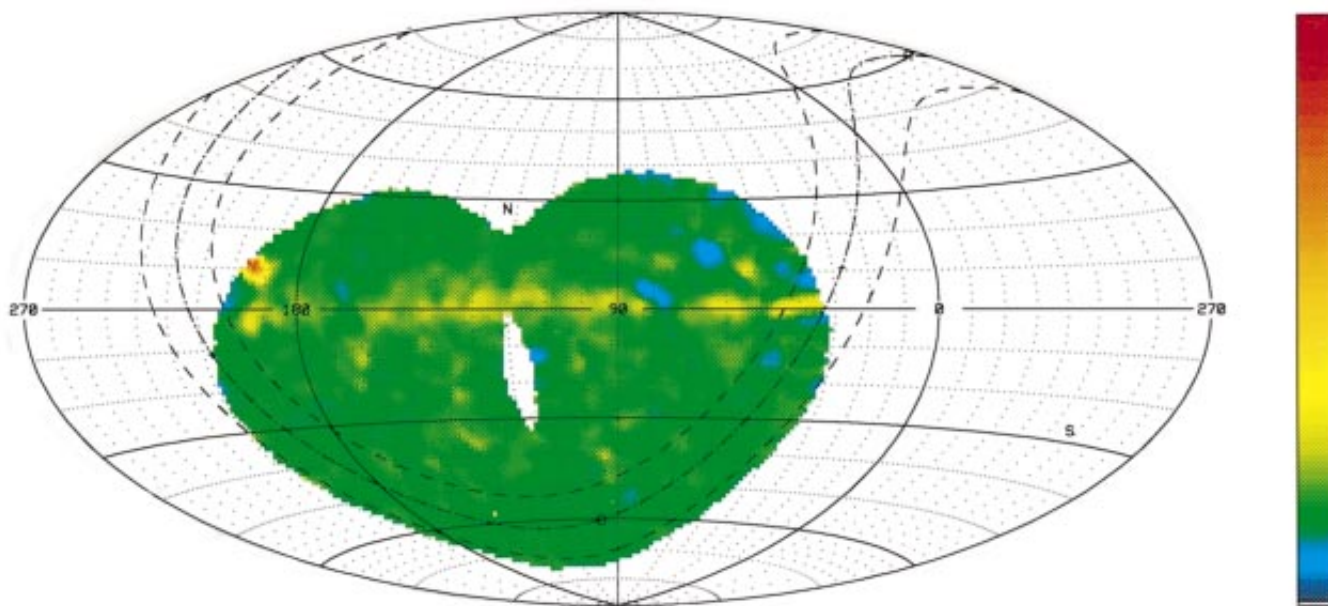
MICROWAVE MAP derived from the M.I.T./Princeton balloon experiment matches observations by the Cosmic Background
